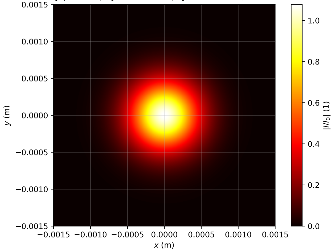
Intensity profile I(x, y, z = 0.557m)/I_0 , Pin=0.6Pcr, artificial time
